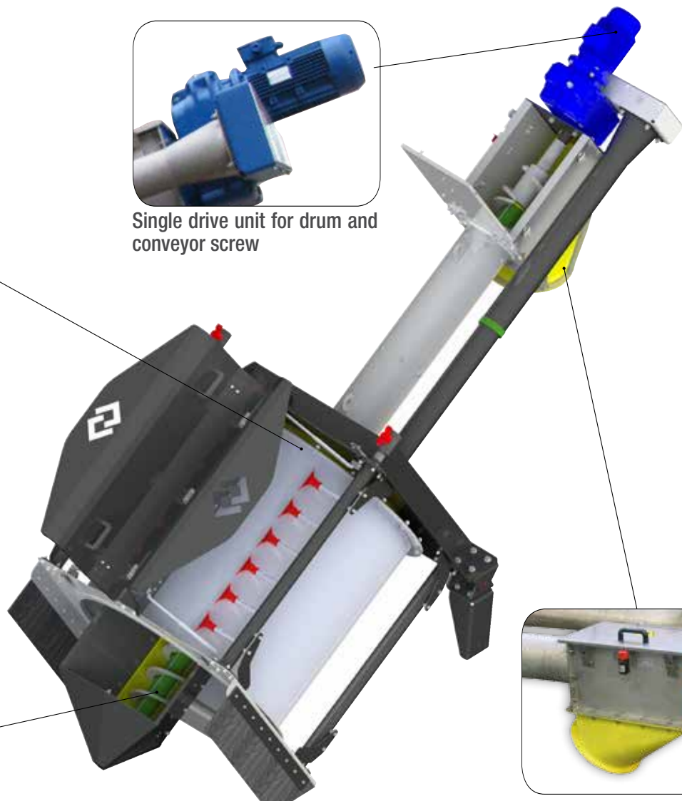
Rotary drum with cleaning nozzles
